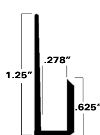
A50-0078 .040 nominal metal thickness
