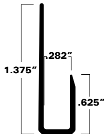
A50-0075 Punched and slotted .050 nominal metal thickness
