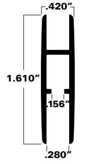
Large Locking Shoe A52-6668
