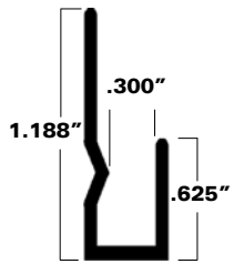
A50-0080 Punched and slotted .050 nominal metal thickness
