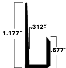
A50-0060 .055 nominal metal thickness
