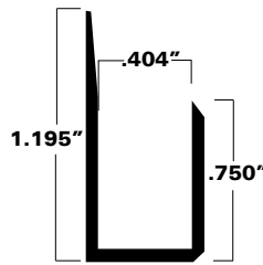
A50-3133 .051 nominal metal thickness
