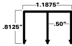
Deep Header Slide Track A54-0372
