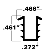
Vinyl Insert for Shoe V25-2500 1/4" glass only
