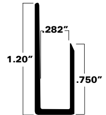
A50-0058 Punched and slotted .050 nominal metal thickness
