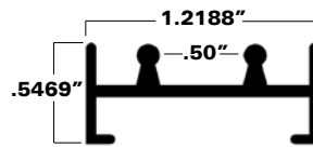
Lower Security Track A54-0371 Glass Deduction = 1.4375"
