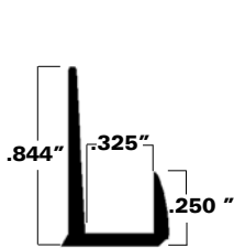
A50-6045 .055 nominal metal thickness
