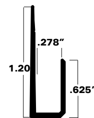
A50-0079 .040 nominal metal thickness
