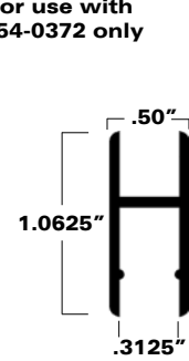
Locking Shoe A52-6303
