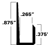
A50-0077 .040 nominal metal thickness
