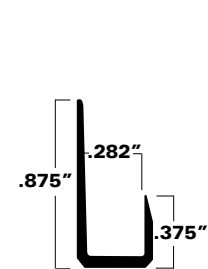
A50-0074 Punched and slotted .050 nominal metal thickness
