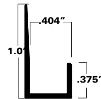
A50-3134 .051 nominal metal thickness
