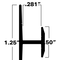
A50-0058 Punched and slotted .050 nominal metal thickness
