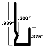
A50-0081 Punched and slotted .050 nominal metal thickness
