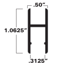
Locking Shoe A52-6303
