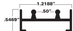
Lower Security Track A54-0371
