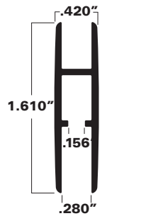
Large Locking Shoe A52-6668
