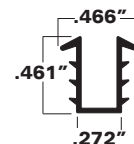
Vinyl Insert for Shoe V25-2500 1/4" glass only
