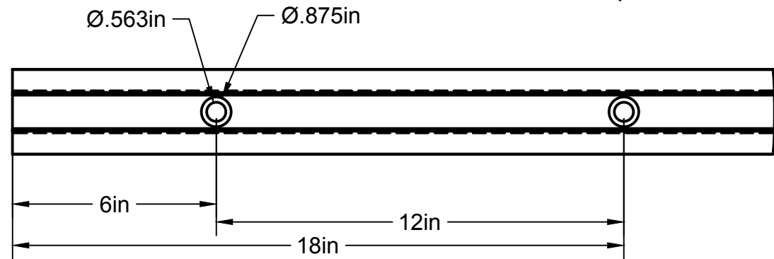
DETAIL A SCALE 1:4
