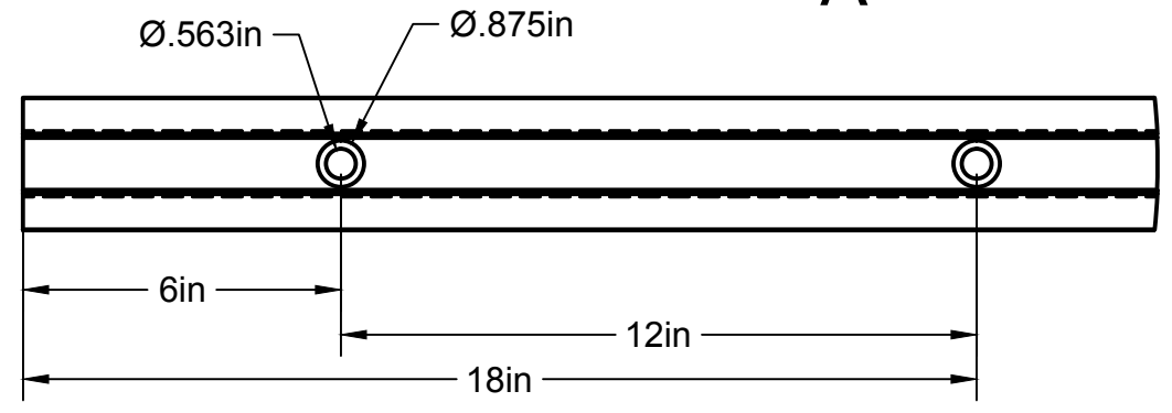
DETAIL A SCALE 1:4
